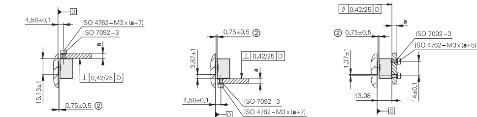
Mounting options for scanning head
