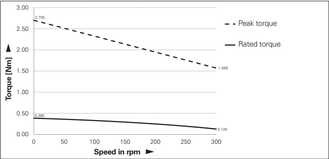
Characteristic curve of torque at DC 48 V
