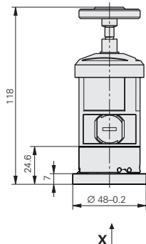
Quick release with magnetic base
