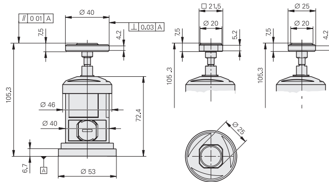
Mounting base
